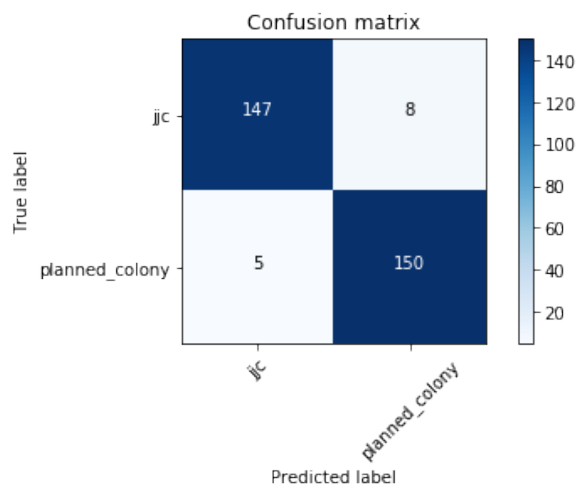
Figure 2: Confusion Matrix for Augmented ResNet-18
